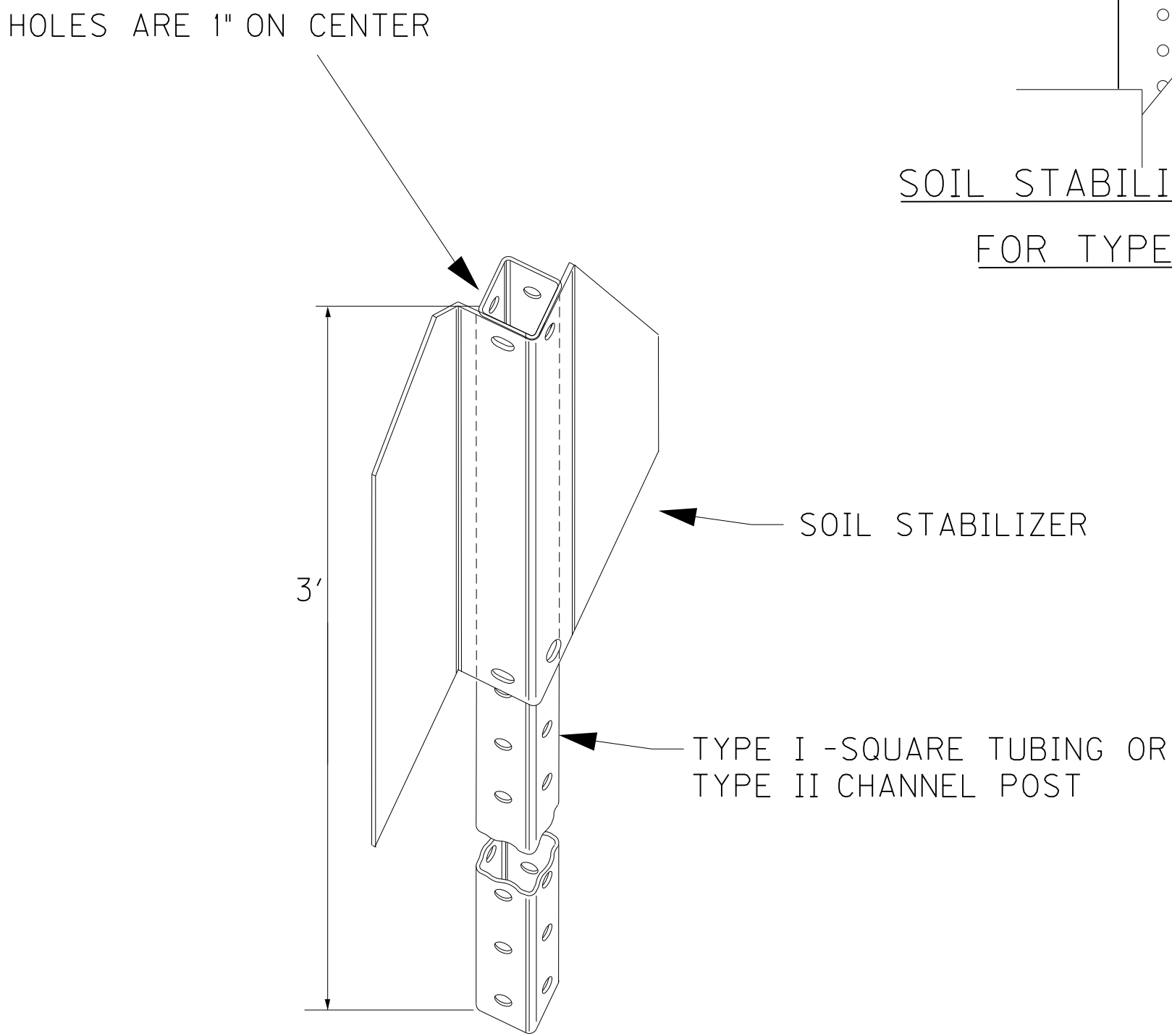
SOIL STABILIZER DETAIL
